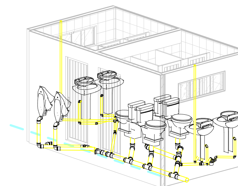
3 3D - BWC'S SOCIAIS
